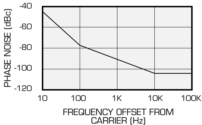
TYPICAL PHASE NOISE CHARACTERISTICS (1.0 Hz BANDWIDTH)
